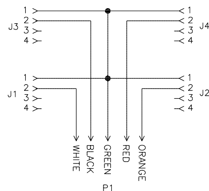
WIRING DIAGRAM
